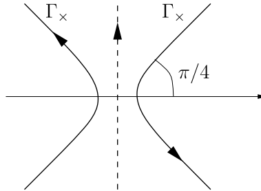
FIG. 4. Integration paths of the Pearcey kernel K_u^{\mathcal{P}} defined in (1.12). The two solid lines form together \Gamma_\times , the dashed line is the z -integration path.
