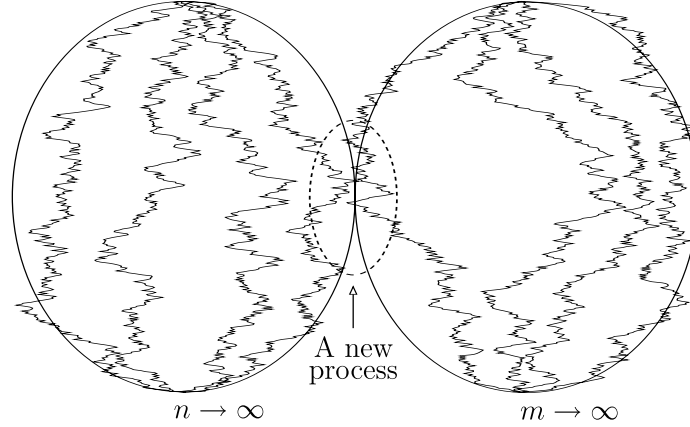
FIG. 5. When two Pearcey cusps touch, there will be a new process.
