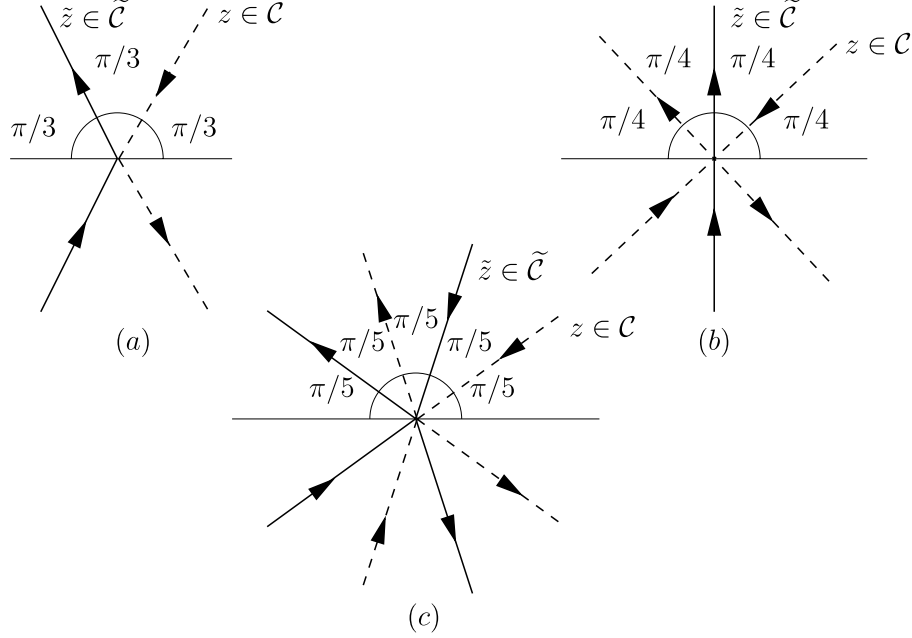
FIG. 7. Integration paths \mathcal{C} (dashed line) and \tilde{\mathcal{C}} (solid line) of the (a) Airy kernel K^A , (b) Pearcey kernel K^P and (c) Quintic kernel K^Q .
