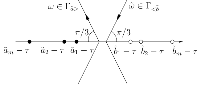
FIG. 2. Integration paths of the kernel K_m^{\tilde{a}, \tilde{b}} of (1.5).
