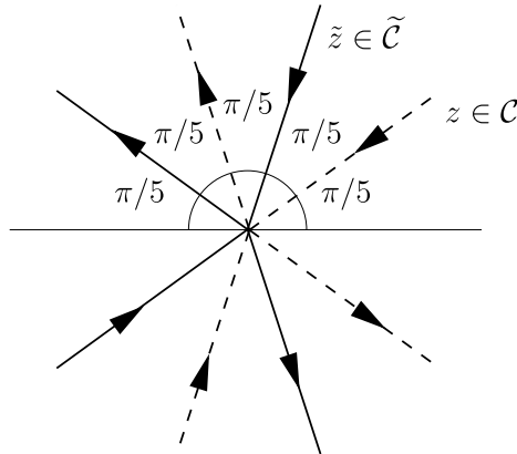
FIG. 6. Integration path \mathcal{C} (dashed line) and \tilde{\mathcal{C}} (solid line) of the quintic kernel.
