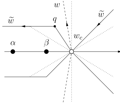
FIG. 10. Second deformation of the previous last contours in Figure 9 for \sigma = \sigma_+ . At the critical point w_c , the path of \tilde{w} has angles \pm\pi/4, \pm3\pi/4 , while the path of w leaves it with any angle in (\pi/2, 3\pi/4) . The value of q will be chosen during the analysis. For \sigma = \sigma_- , one picks the mirror image of the figure above about the vertical line through w_c , with w and \tilde{w} also flipped; that is, the dashed and solid lines are interchanged.
