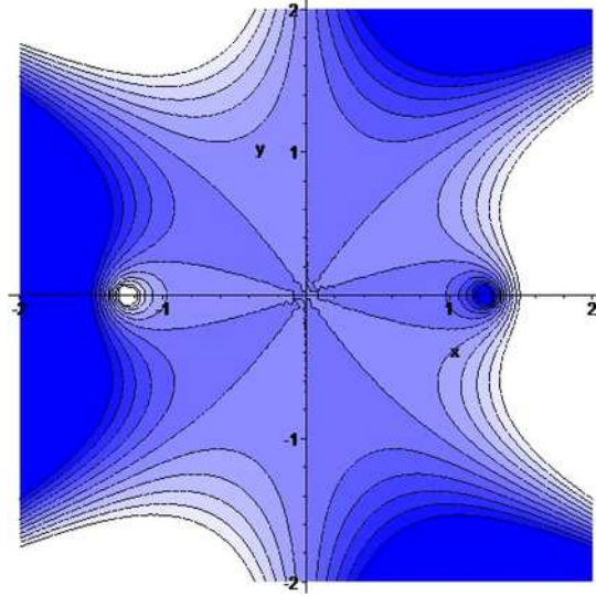
FIG. 13. Contourplot of the function \text{Re}(F(x + iy) - F(0)) . The value is high in dark regions and low in light regions.
